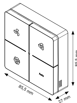
38443 - CO 2 sensor with controls - wall-mounted
