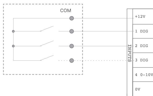
External switch
