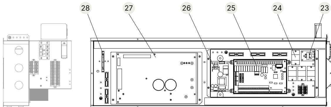
Exploded diagram of electrical box structure
