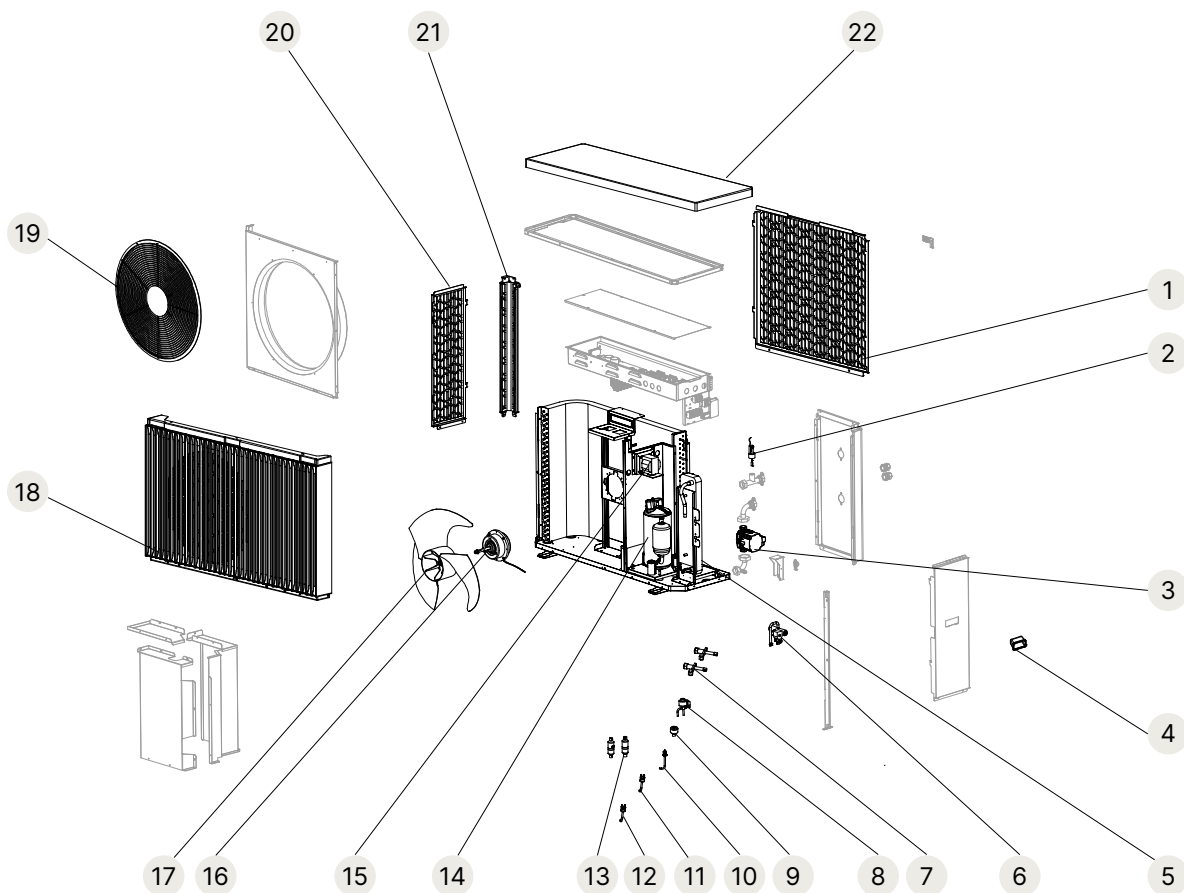
Exploded diagram of complete machine structure
