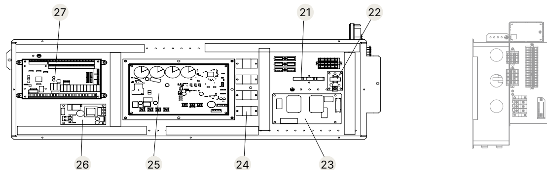
Exploded diagram of electrical box structure
