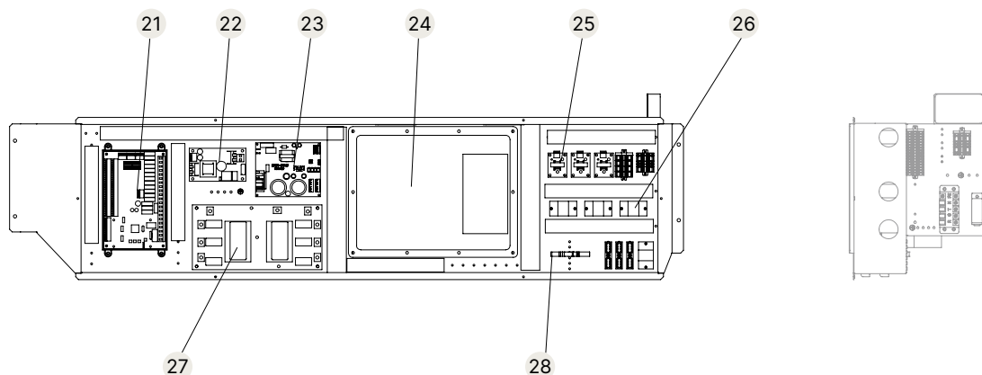
Exploded diagram of electrical box structure
