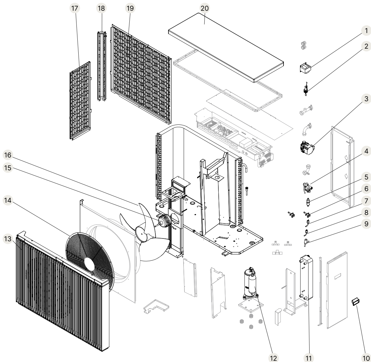
Exploded diagram of complete machine structure
