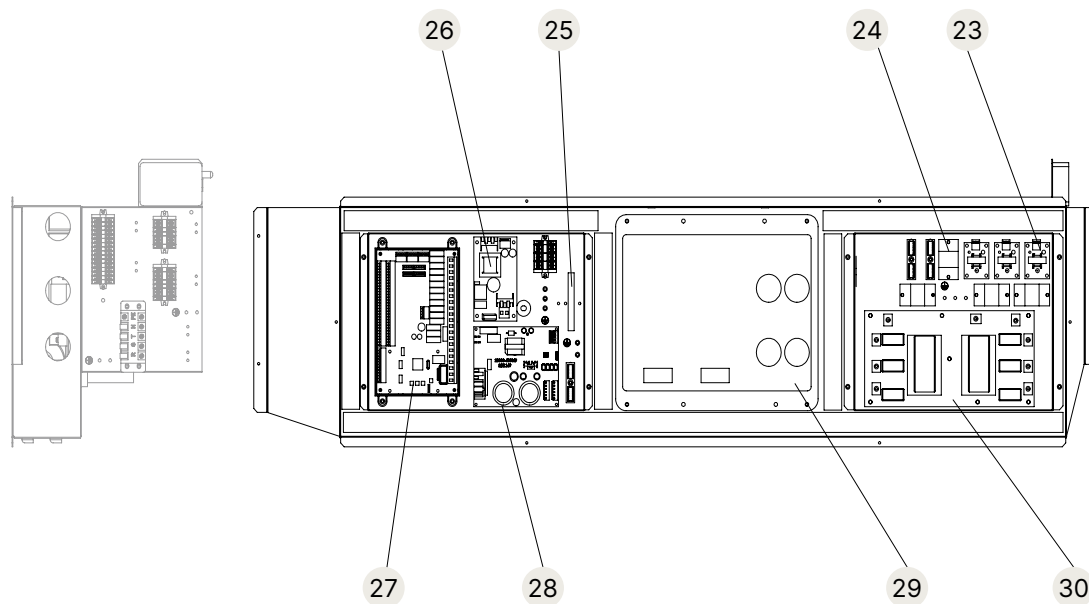
Exploded diagram of electrical box structure
