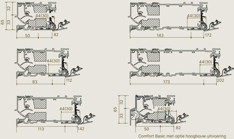
Detailweergave Invisivent® Comfort Basic
