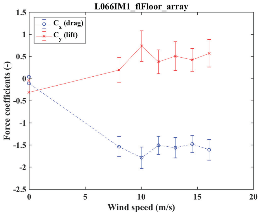
Figure 41: L066IM1 flFloorarray
