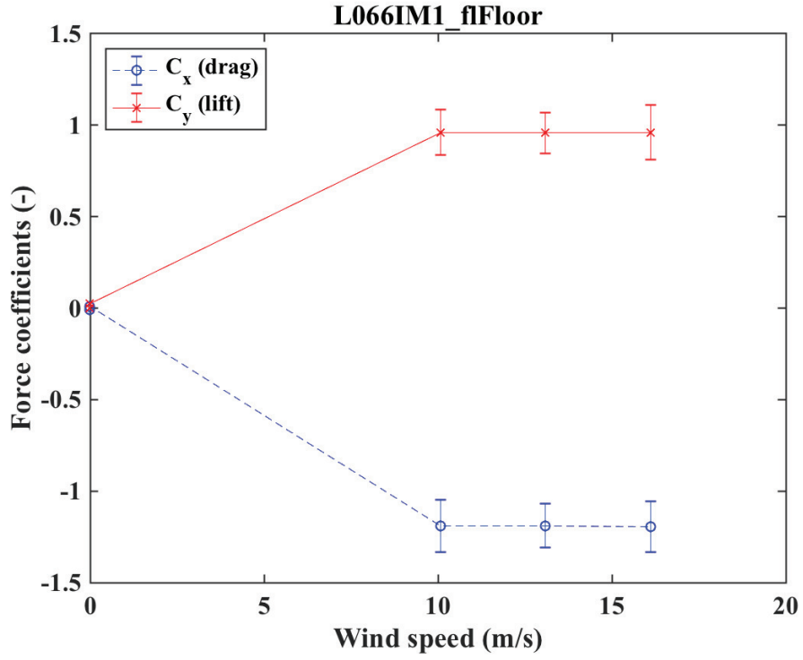
Figure 40: L066IM1 flFloor
