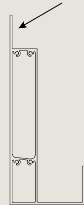
Basic profile variant with wall connection profile
