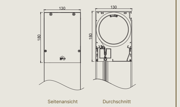
Large – EW 7B – Kassette
