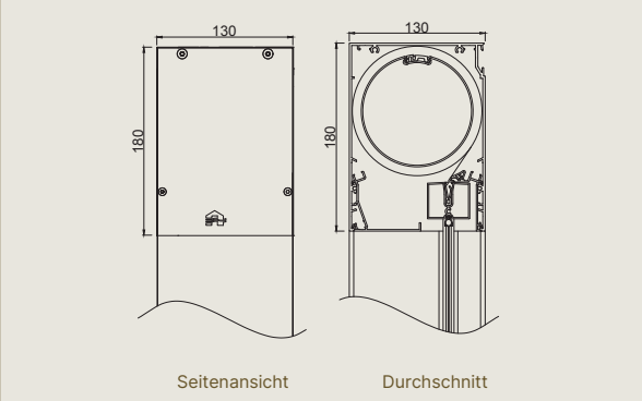
Large – EW 7A – Kassette
