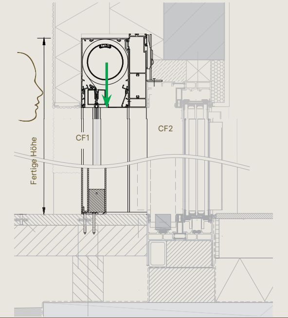
Medium – EW 7B – Kassette
