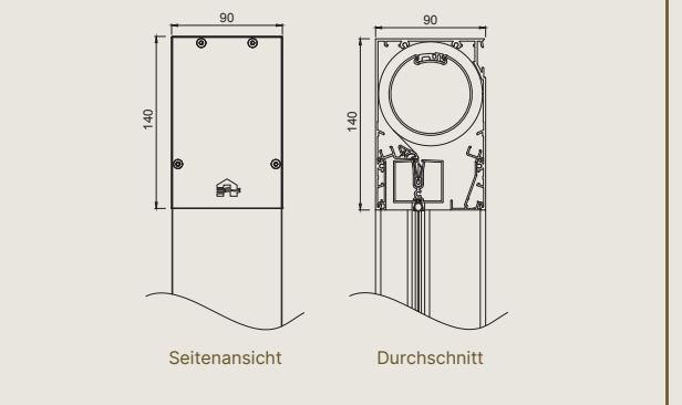
Medium – EW 7B – Kassette
