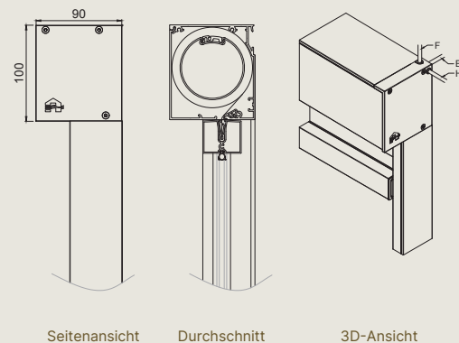
Small – Kassette
