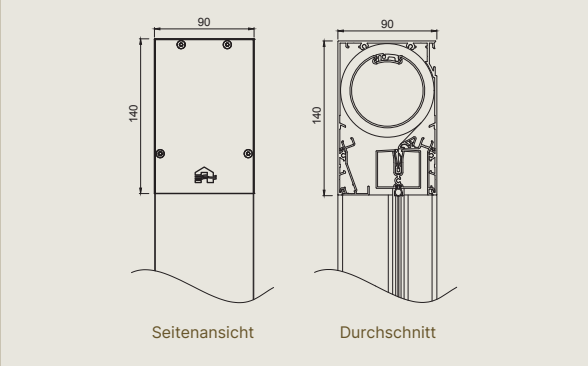
Medium – EW 7A – Kassette
