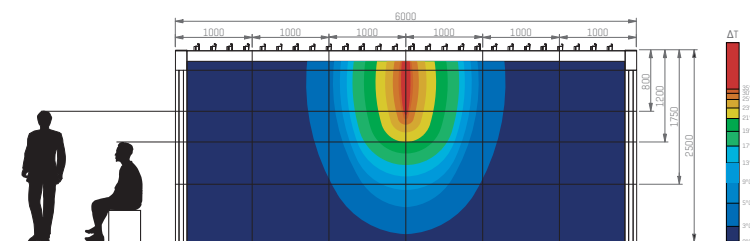
1 Lineo heat blade with 1 heater
