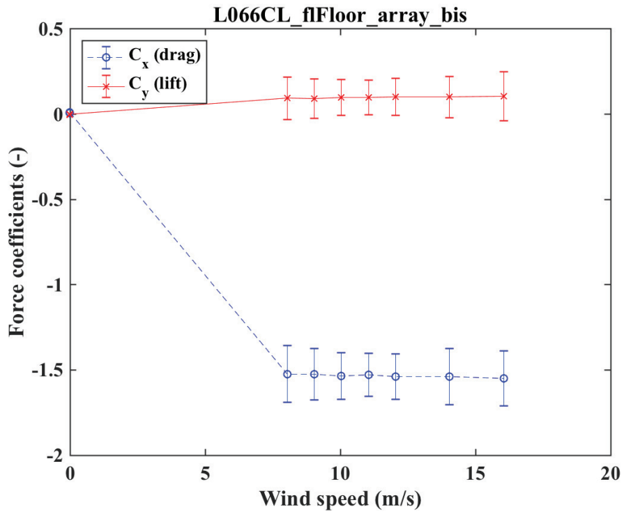
Figure 39: L066CL flFloorarraybis
