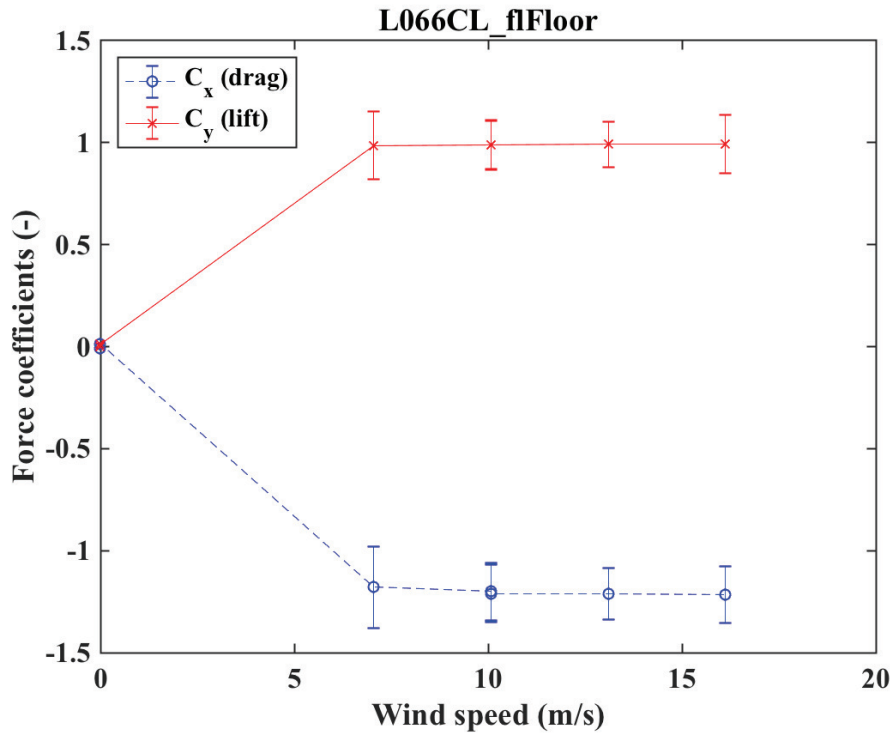
Figure 38: L066CL flFloor
