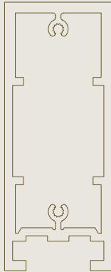
Ref. SD.100 Grote vrije overspanning
